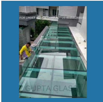
Laminated 11.52mm (5mm Glass -1.52mm PVB-5mm Glass) Laminated Glass
